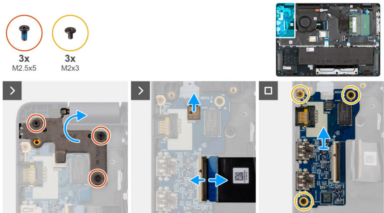
Abbildung 38. Removing the I/O board
