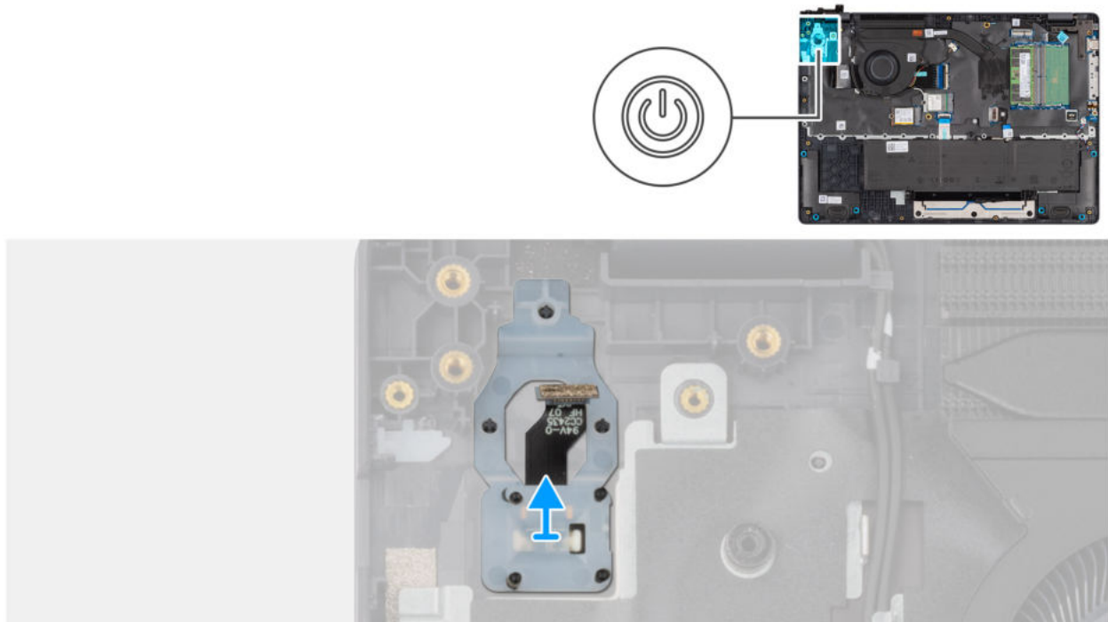
Abbildung 44. Removing the power button with fingerprint reader
