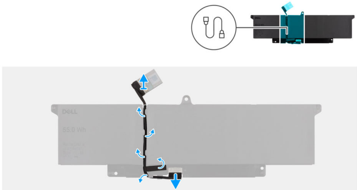
Abbildung 19. Removing the battery cable
