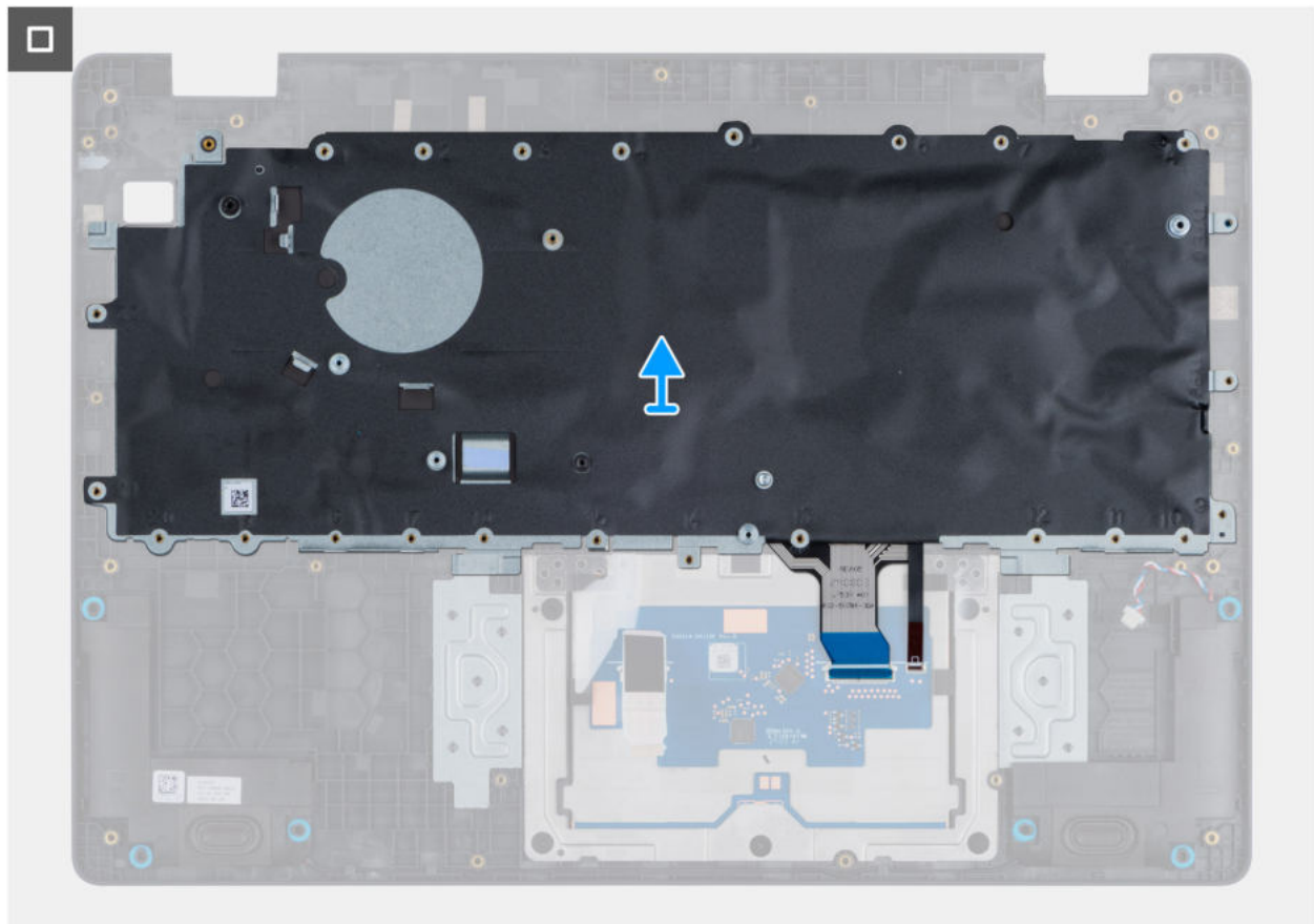
Abbildung 61. Removing the keyboard
