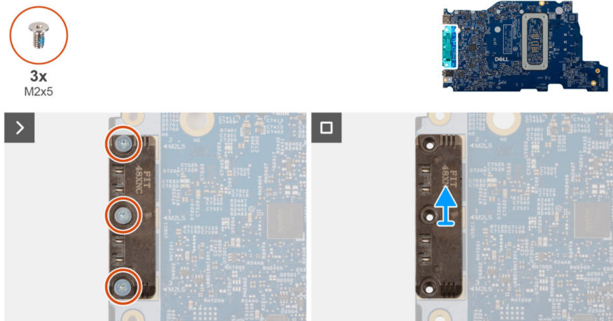
Abbildung 58. Removing the USB Type-C module
