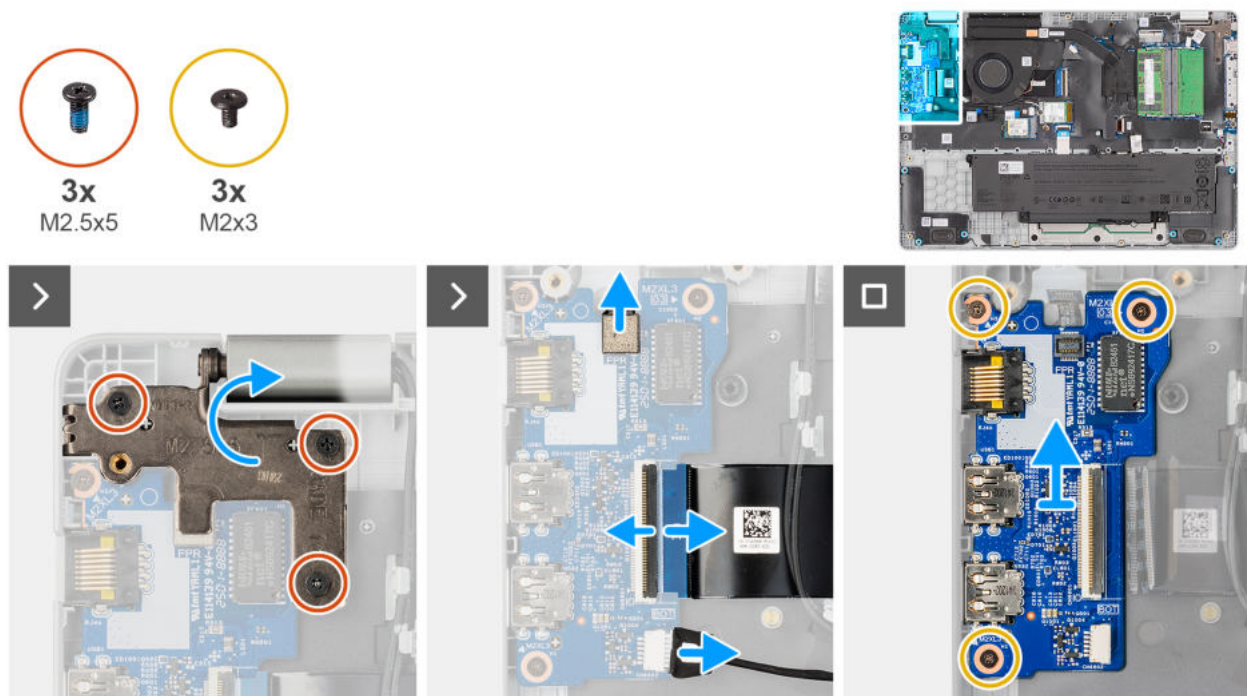
Abbildung 40. Removing the I/O board
