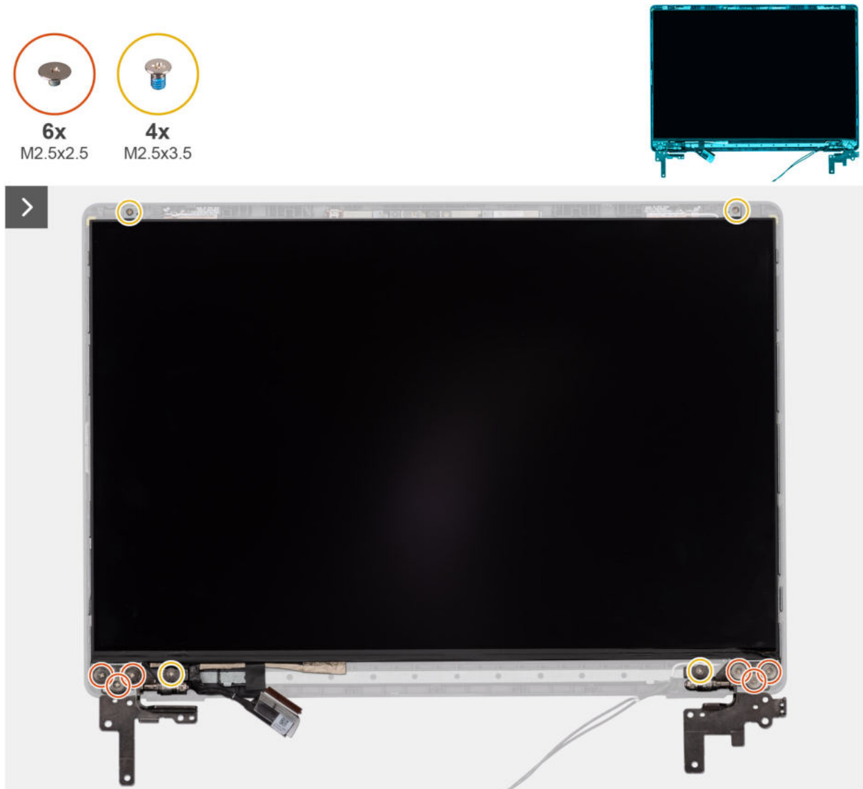
Abbildung 84. Removing the display-panel assembly
