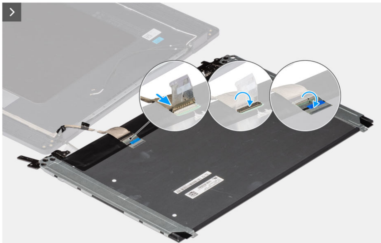
Abbildung 89. Installing the display-panel assembly
