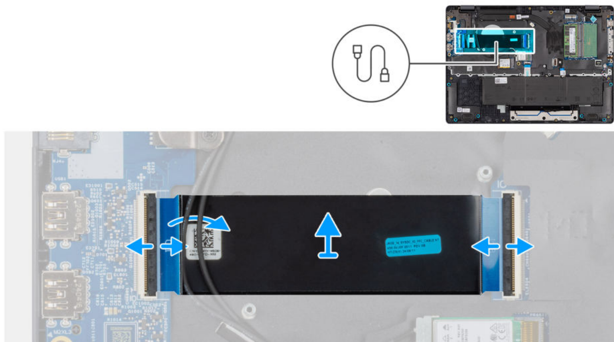
Abbildung 42. Removing the I/O-board FPC cable
