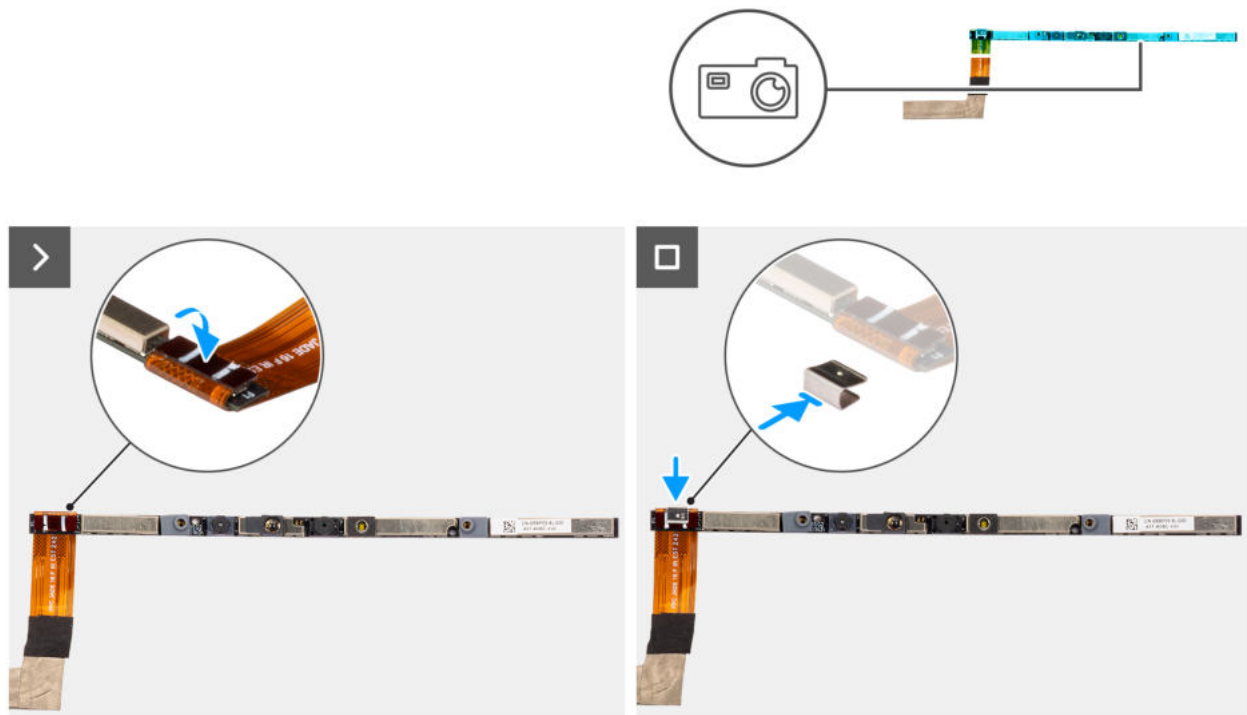
Abbildung 93. Installing the camera
