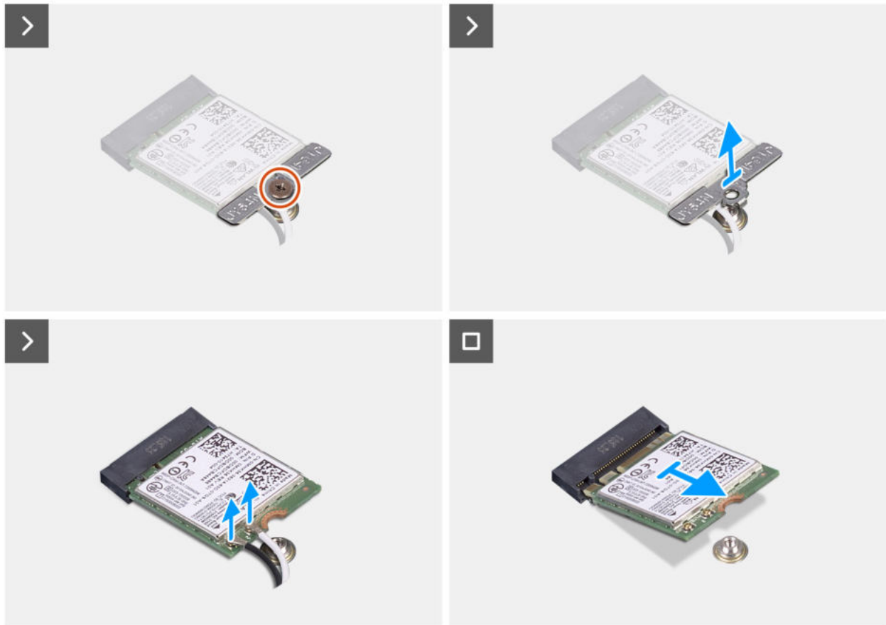
Abbildung 25. Removing the wireless card
