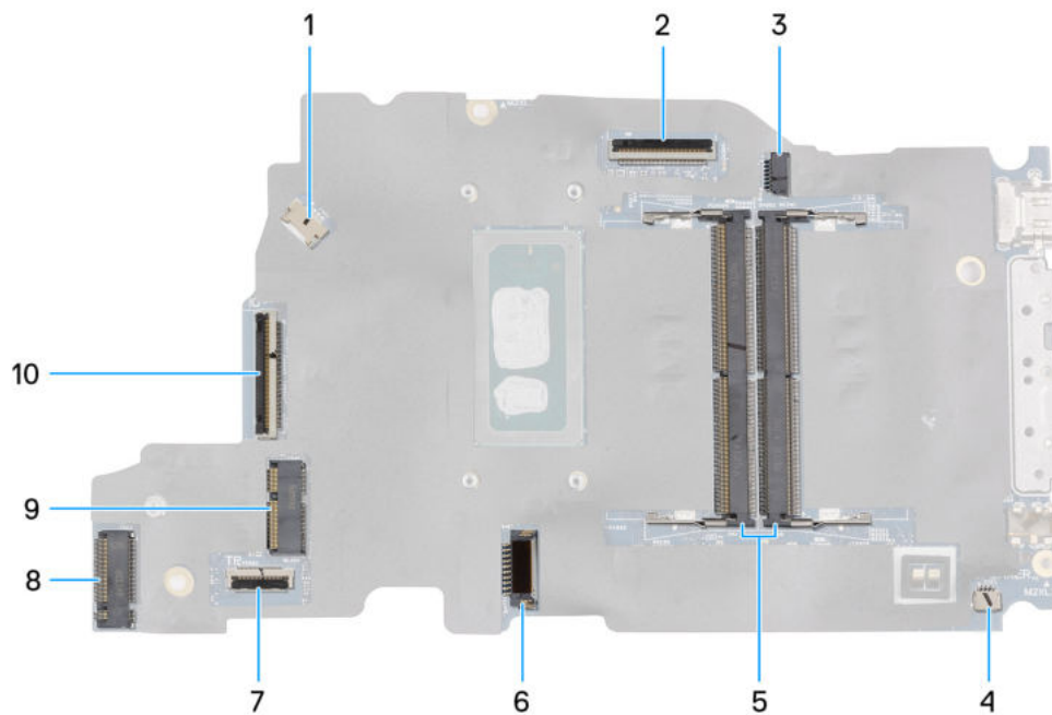
Abbildung 49. System-board connectors
