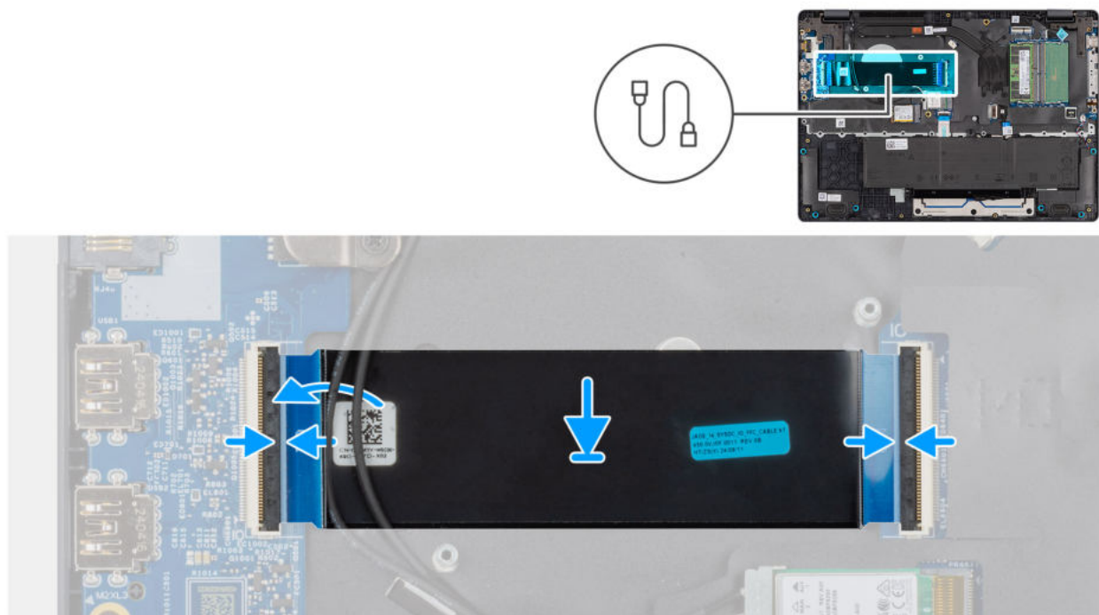
Abbildung 43. Installing the I/O-board FPC cable
