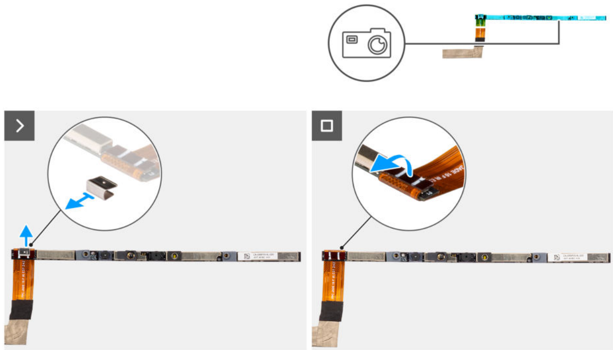
Abbildung 92. Removing the camera
