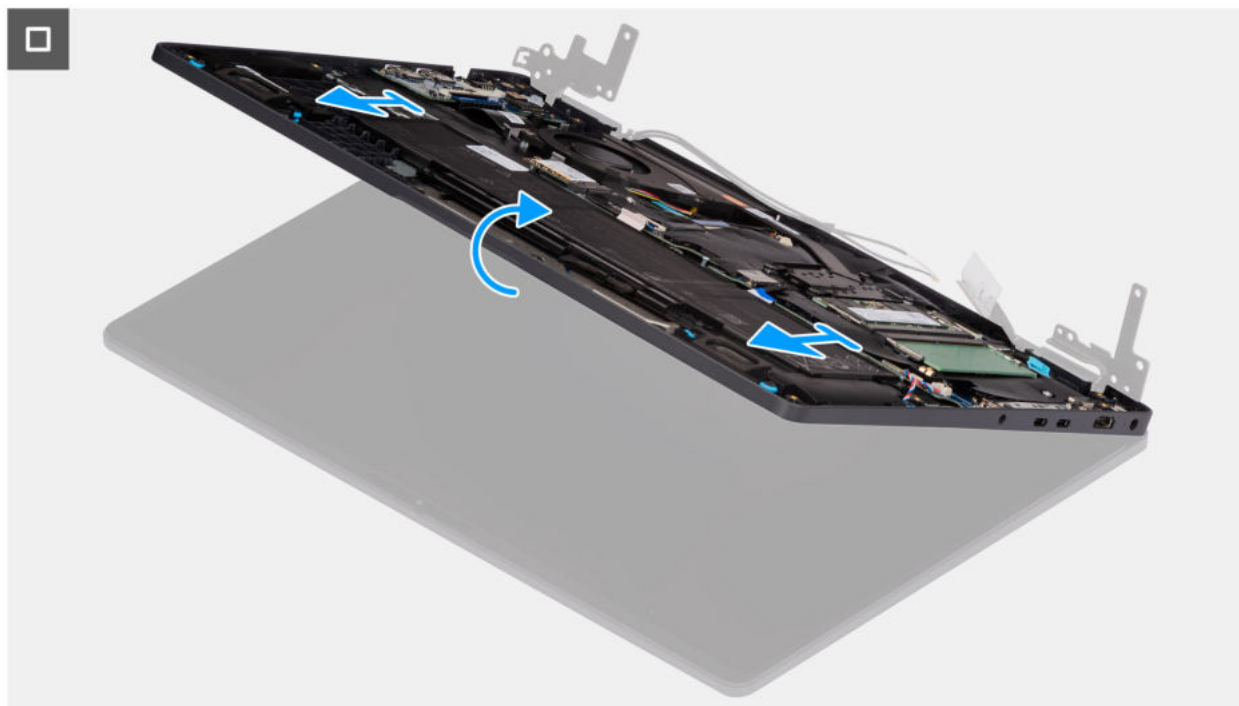
Abbildung 73. Removing the display assembly
