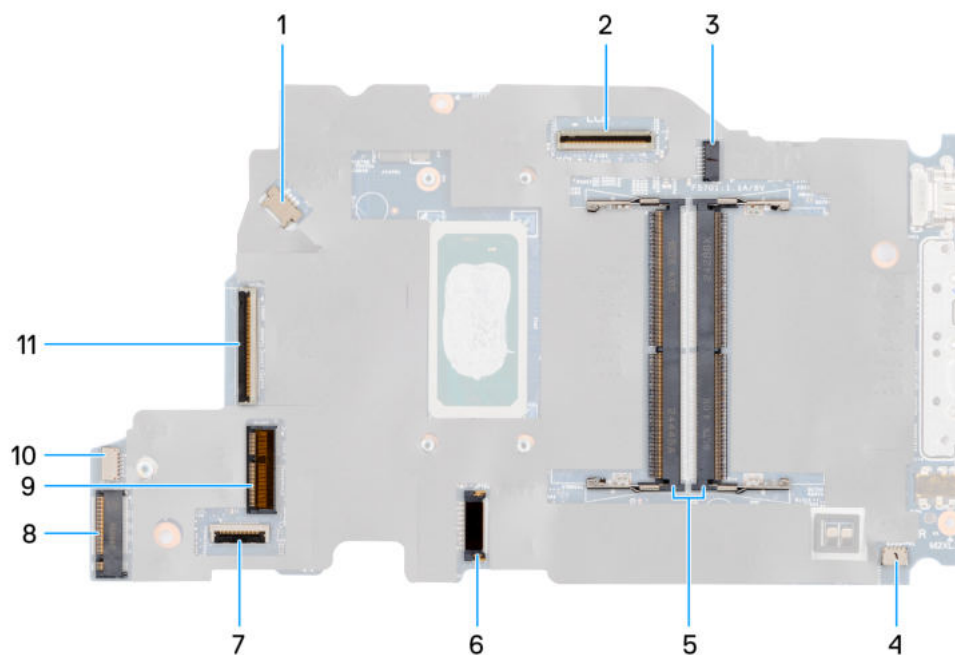
Abbildung 52. System-board connectors
