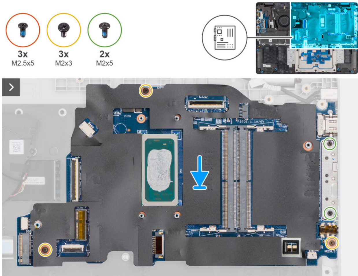
Abbildung 56. Installing the system board
