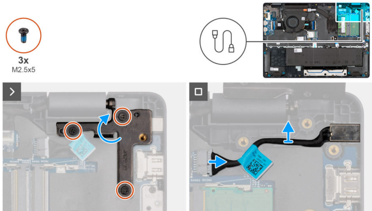
Abbildung 32. Removing the power-adapter port
