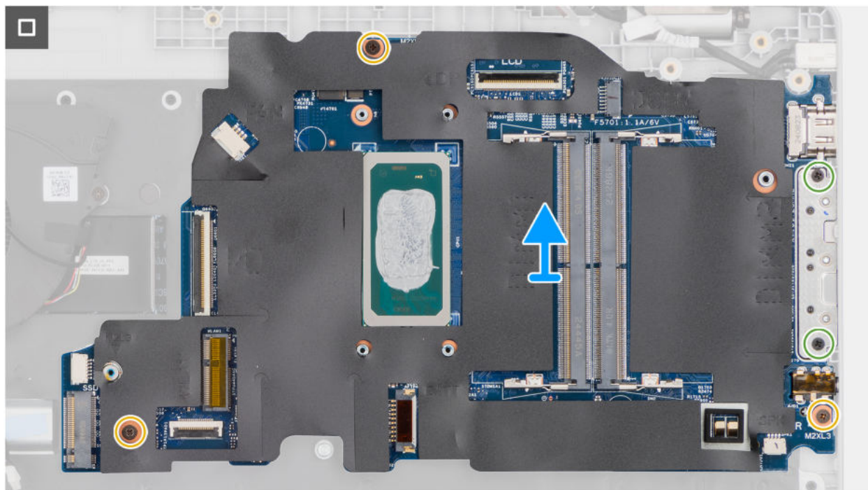
Abbildung 54. Removing the system board
