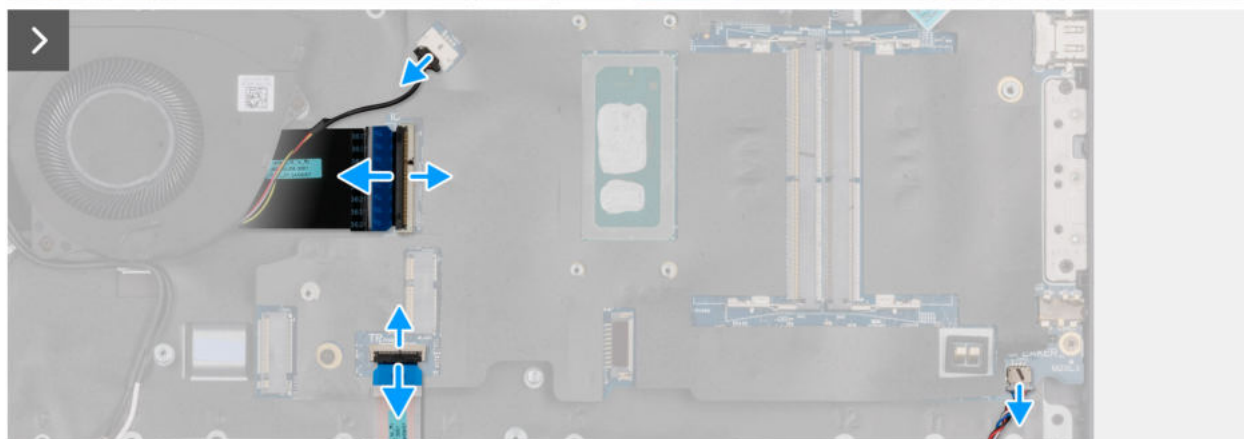
Abbildung 47. Removing the system board
