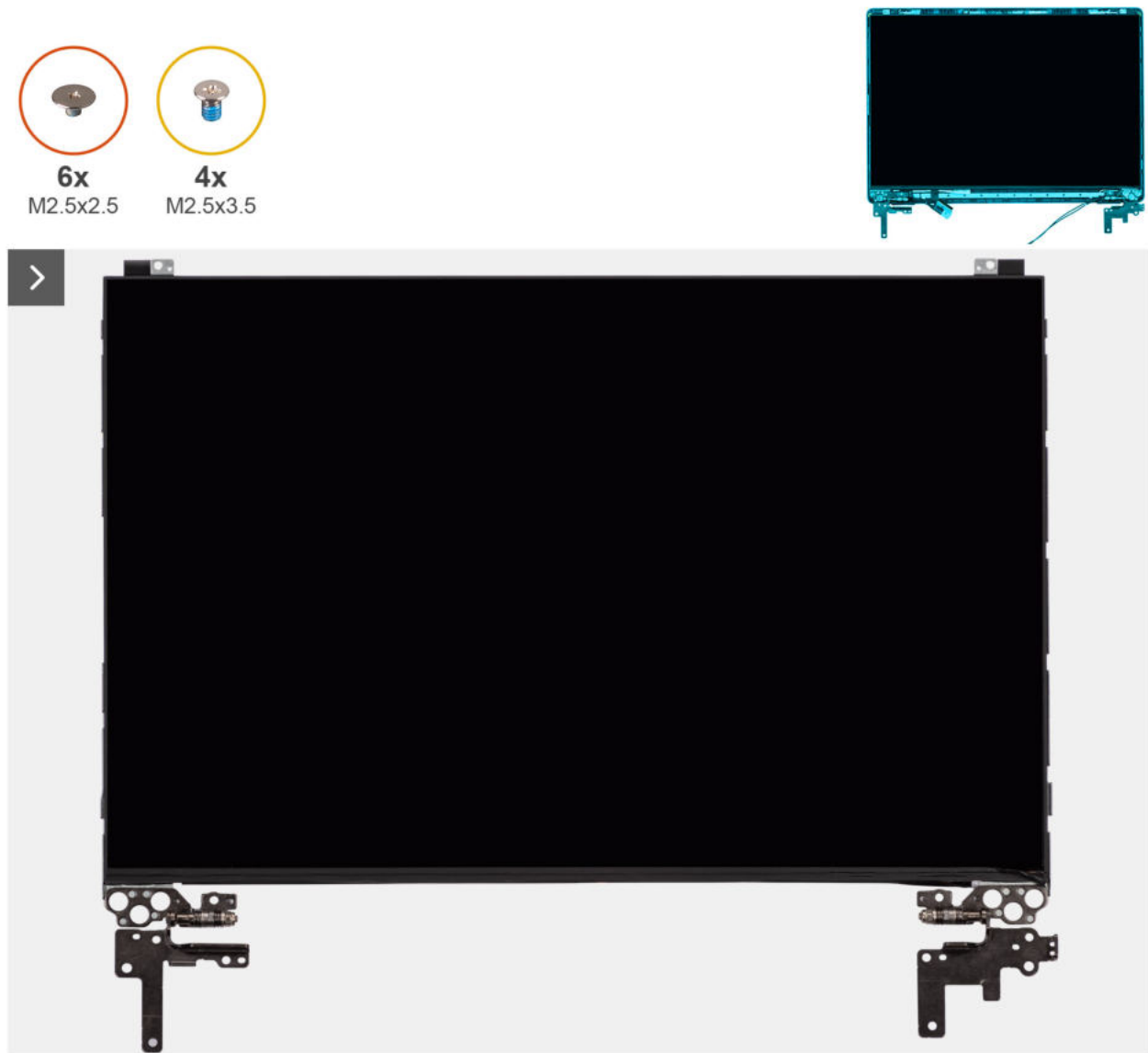
Abbildung 88. Installing the display-panel assembly
