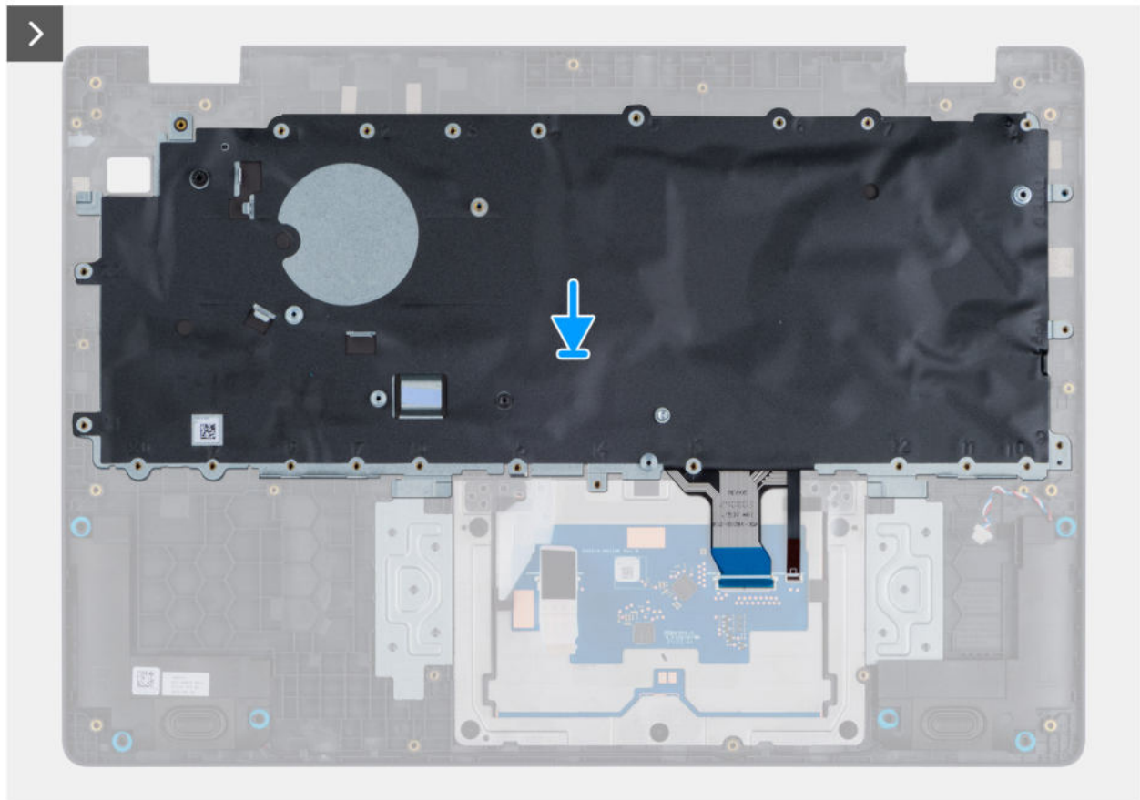
Abbildung 64. Installing the keyboard
