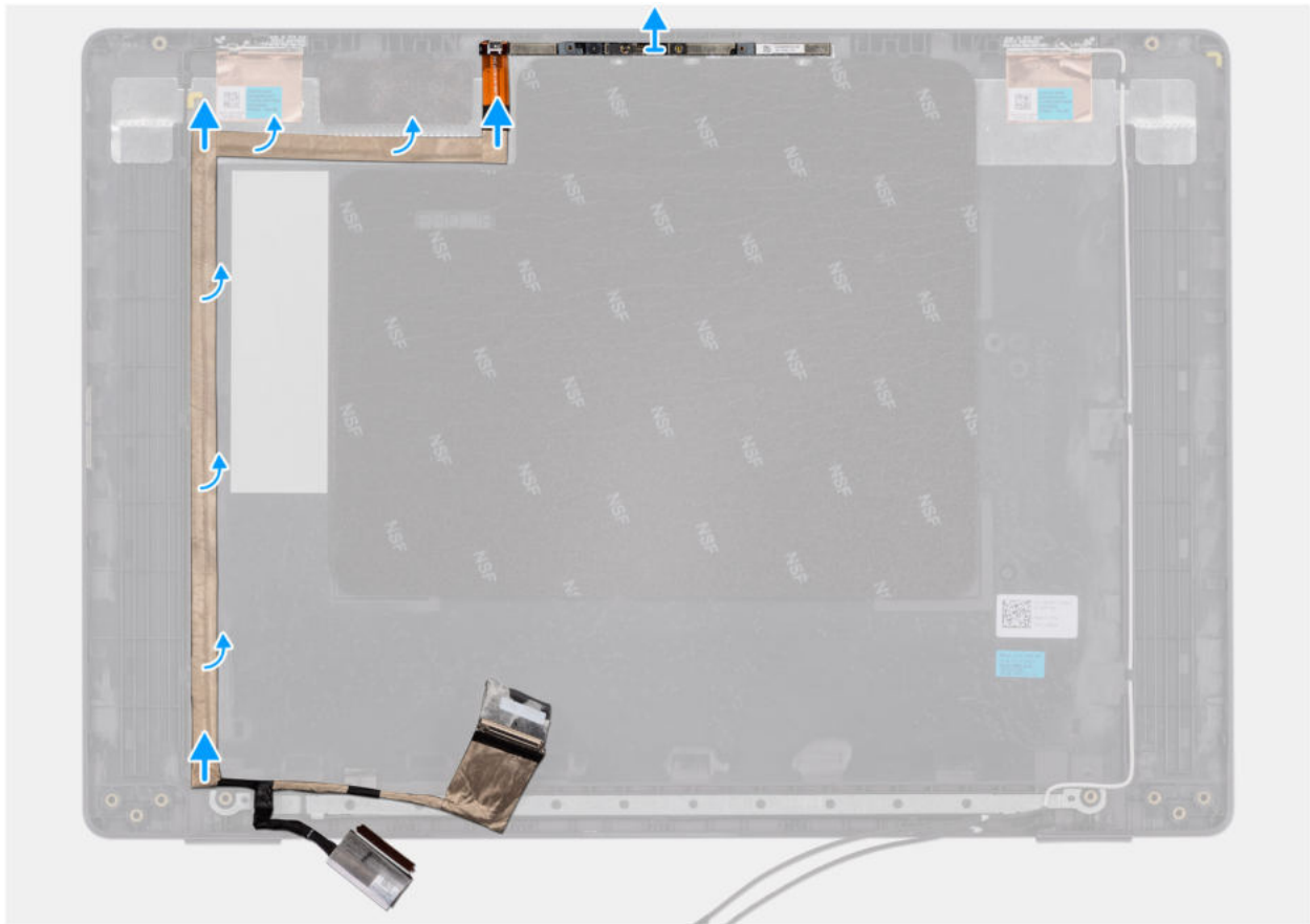
Abbildung 94. Removing the eDP cable
