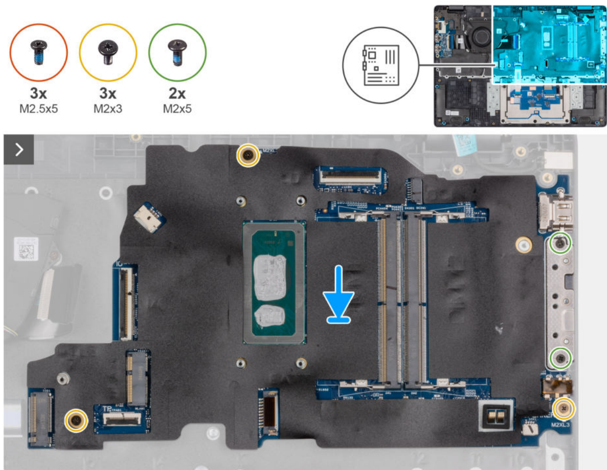
Abbildung 50. Installing the system board
