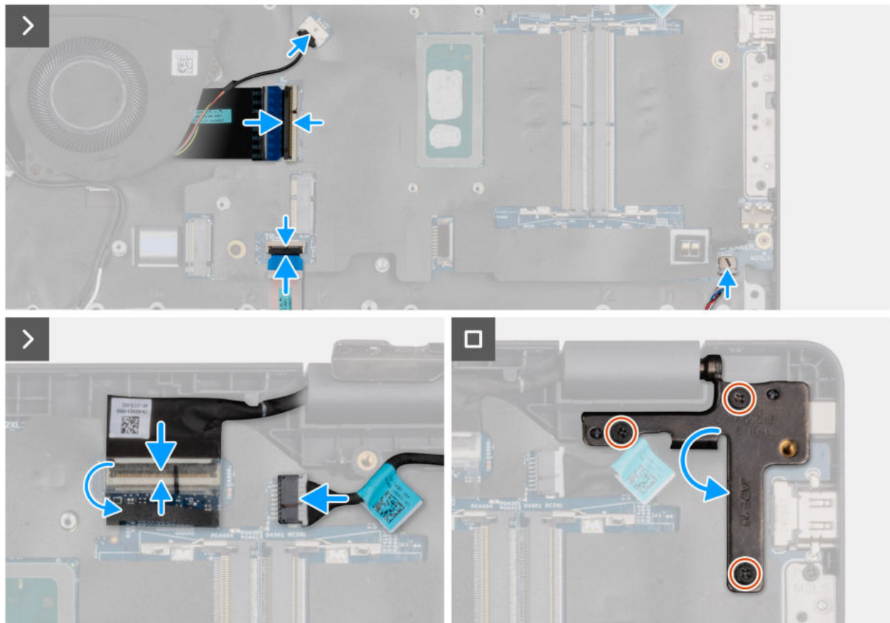
Abbildung 51. Installing the system board
