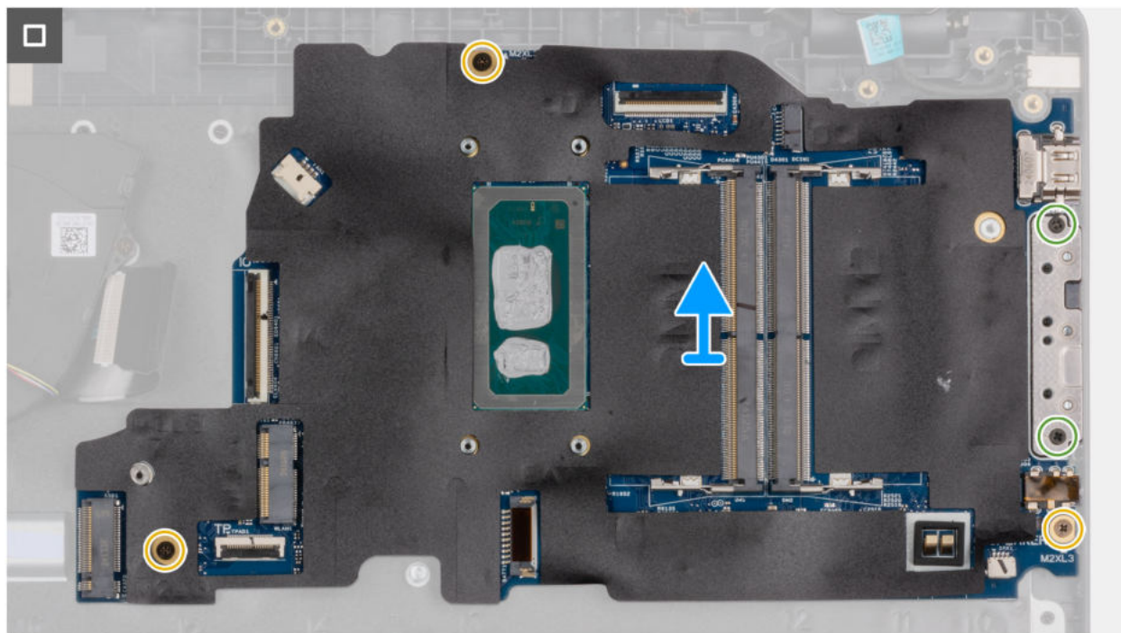
Abbildung 48. Removing the system board
