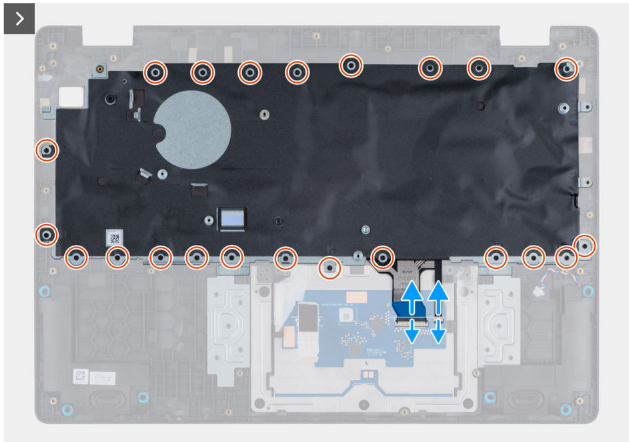
Abbildung 60. Removing the keyboard
