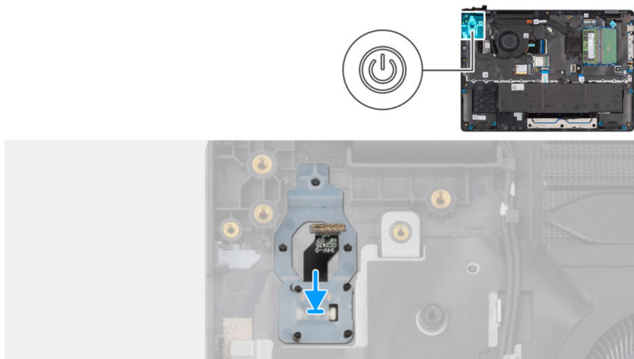
Abbildung 45. Installing the power button with a fingerprint reader
