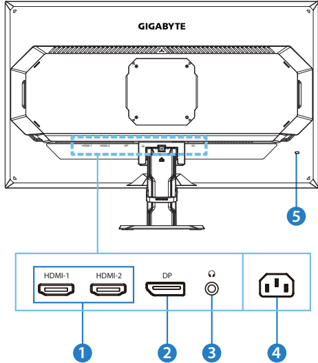
1 HDMI-Anschlüsse (x2)
