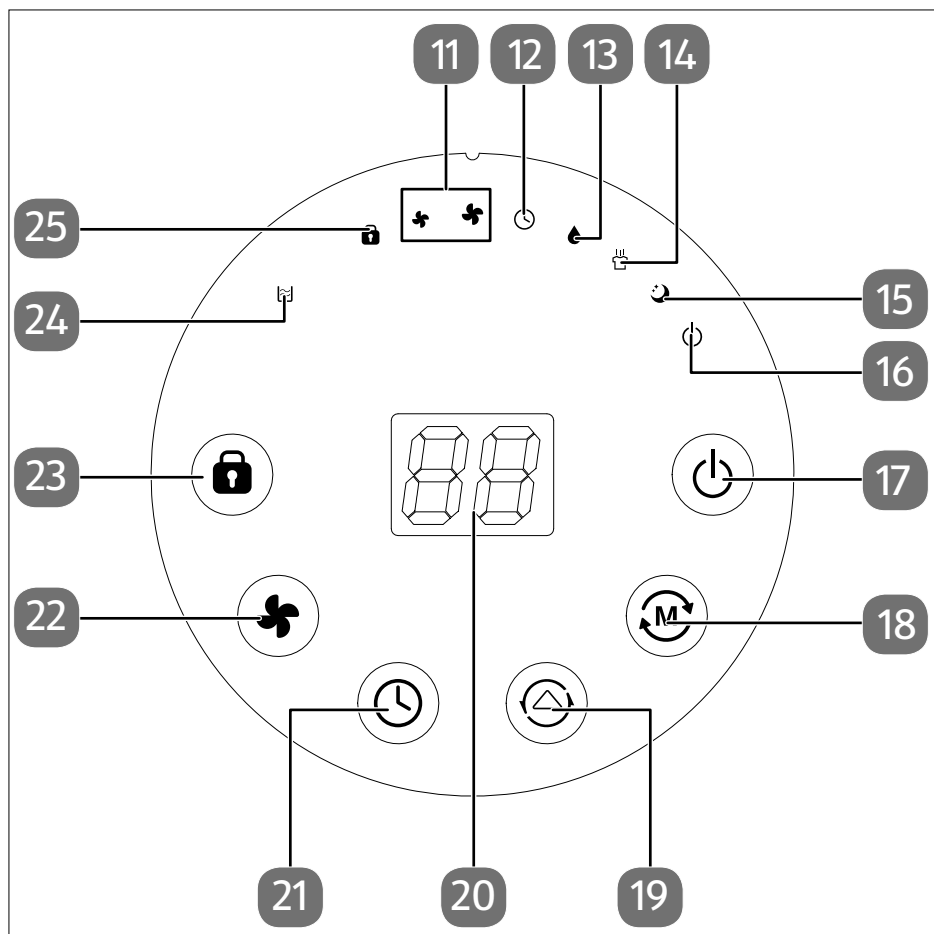
Fig. 3 – Panel de control
