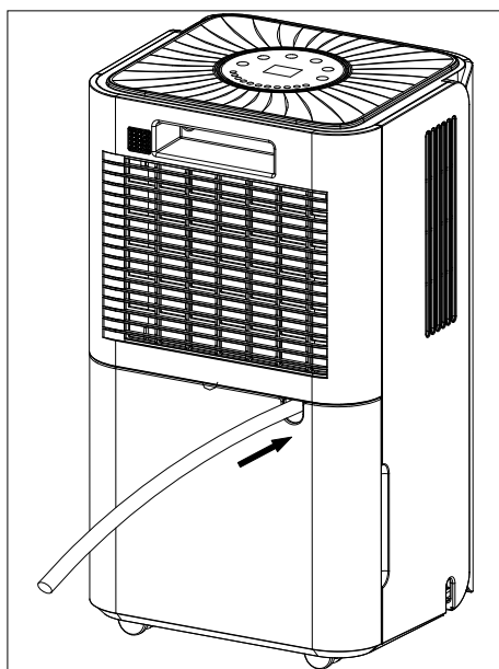
Fig. 5 – Attaching the condensate hose
