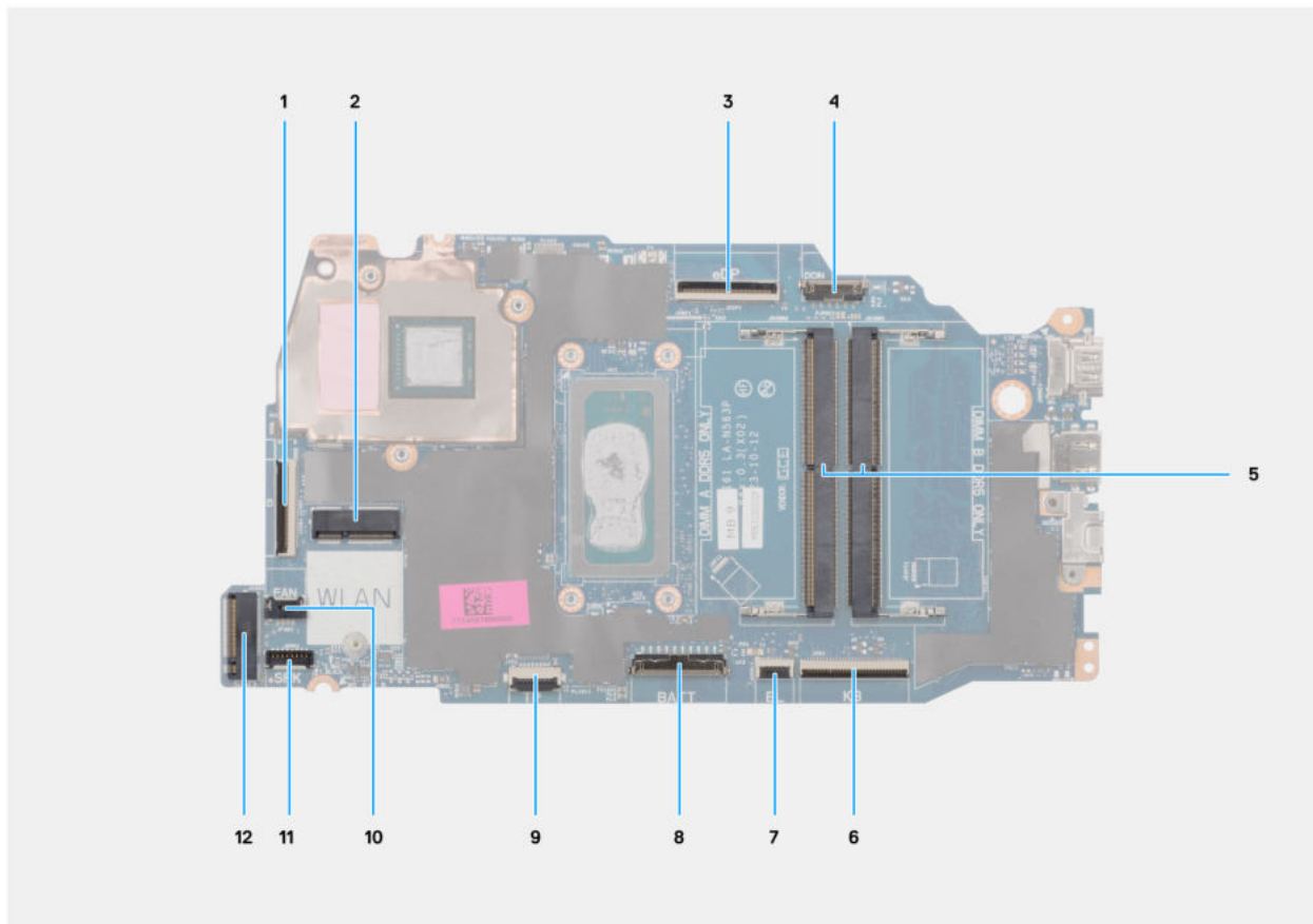
Abbildung 79. System board connectors
