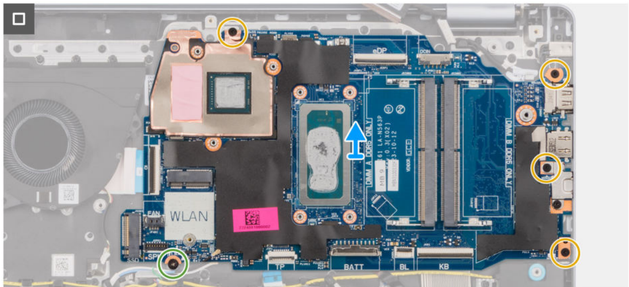
Abbildung 82. Removing the system board
