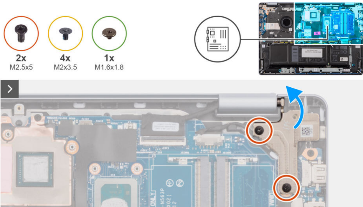
Abbildung 80. Removing the system board
