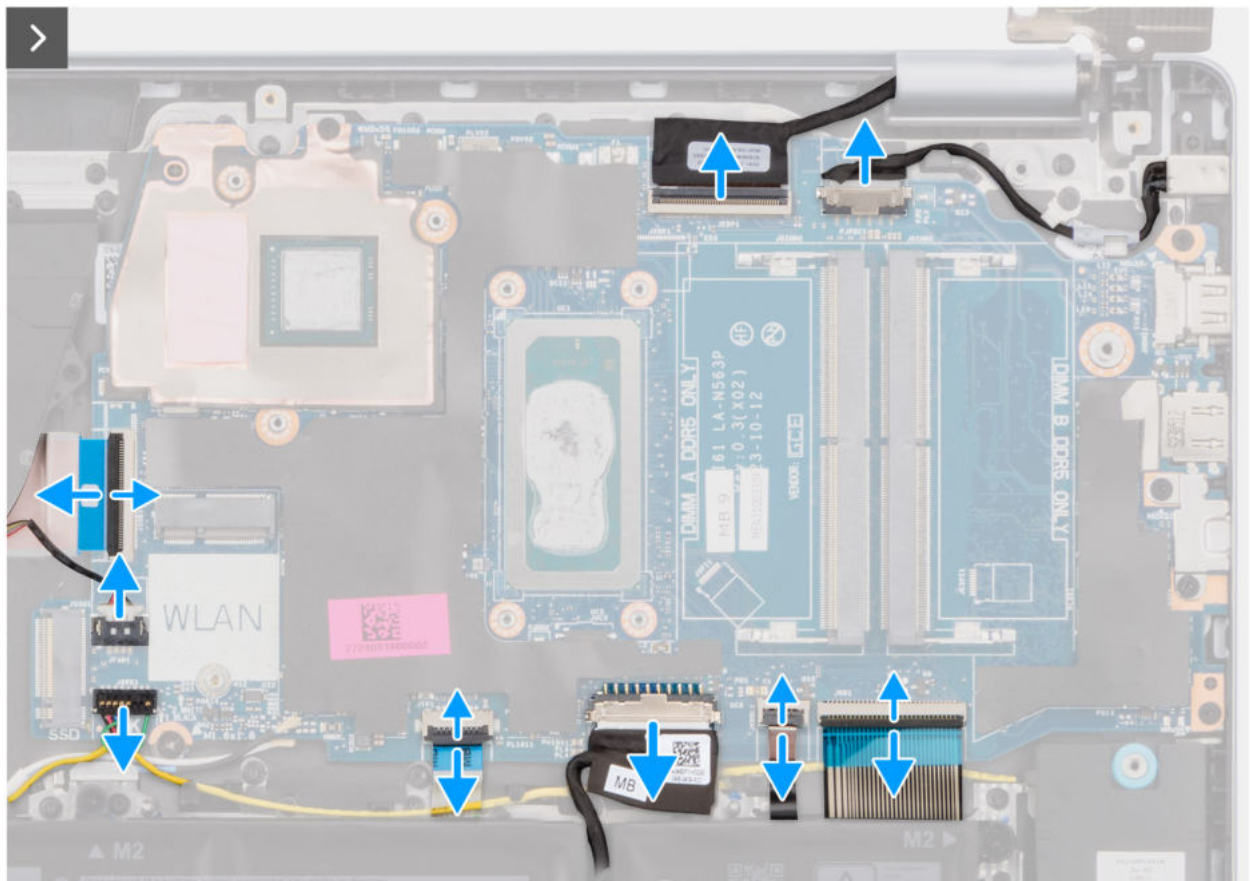
Abbildung 81. Removing the system board
