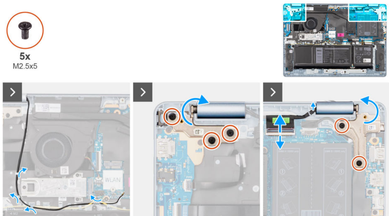
Abbildung 50. Removing the display assembly
