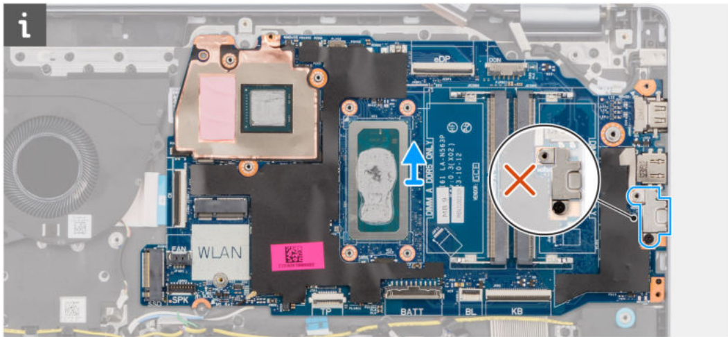
Abbildung 83. System board - USB Type-C bracket
