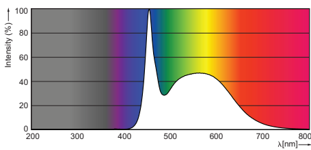
LEDtube HF 1200mm HO 18 W /865 T8 ROT
